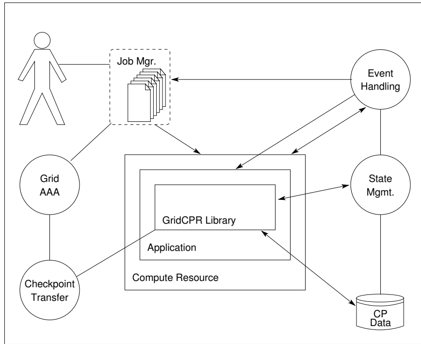
Figure 1: GridCPR Component and Workflow Diagram
