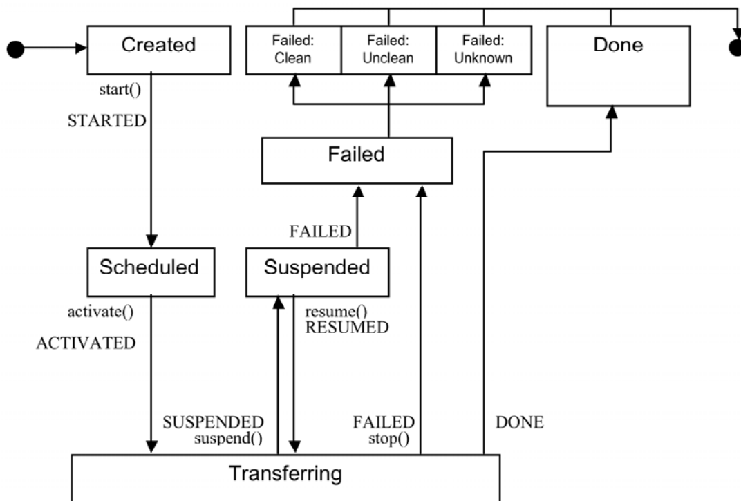
Figure 4: DTI state diagram showing "operations()" and "EVENTS"
