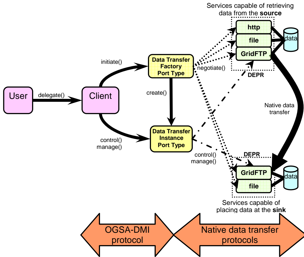
Figure 1: OGSA-DMI Architecture
