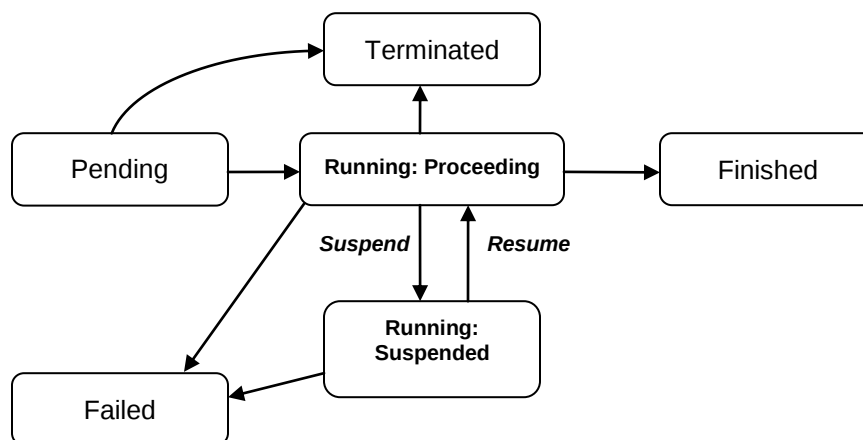
Figure 4. Suspend/resume specialization profile: Activities can be suspended and resumed as a result of appropriate client requests.
