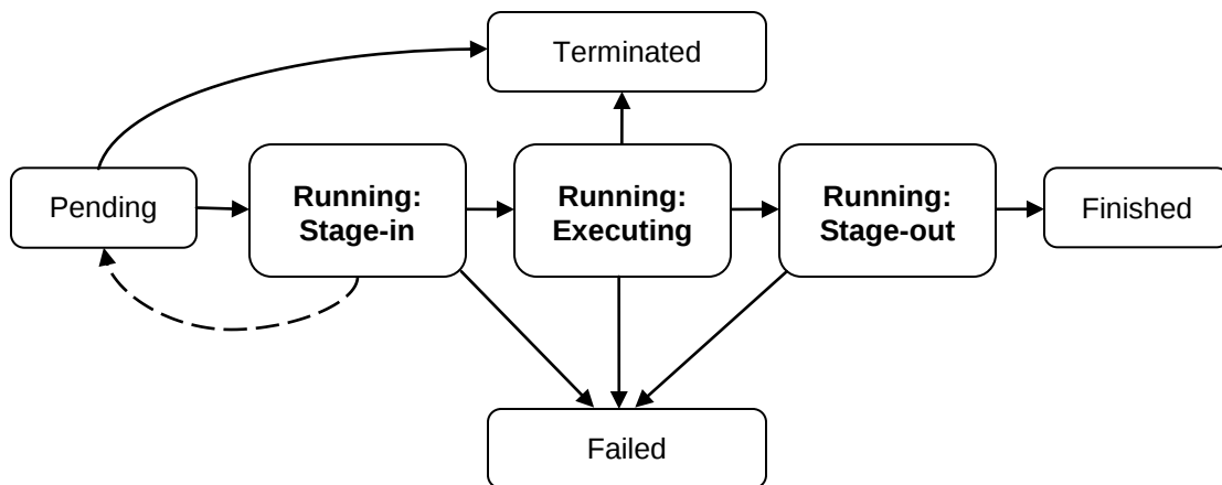
Figure 3. An illegal variation of a data staging specialization profile: Failed data stage-ins result in an activity being placed in the “Pending” state. This profile is illegal because it adds a state transition that would be unexpectedly visible to clients who only understand the basic state model.
