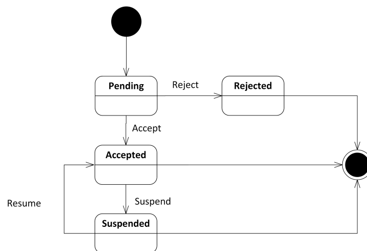
Figure 2. State diagram for Agreement instance, inspired by WS-Agreement states [?] .
