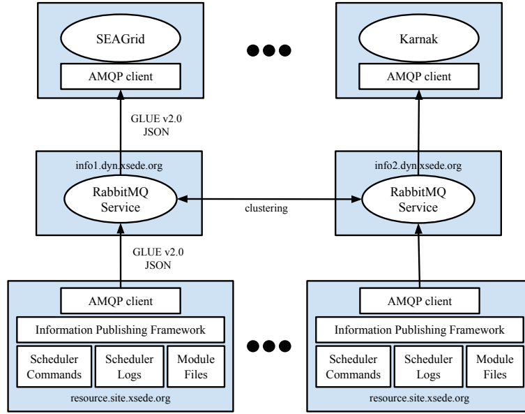
Figure 1: The XSEDE publish/subscribe messaging architecture with GLUE v2.0 information.
