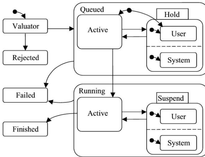
Figure 1: DRMAA Job State Transition Diagram
