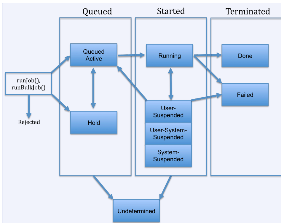
Figure 1: DRMAA Job State Transition Diagram
