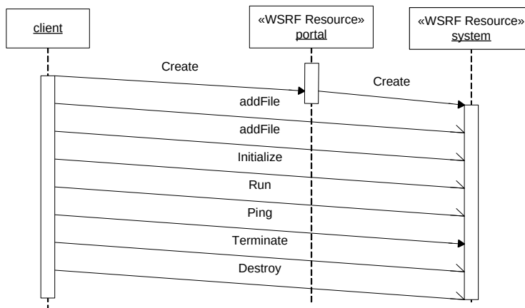
Figure 4. Sequence diagram of a simple deployment
